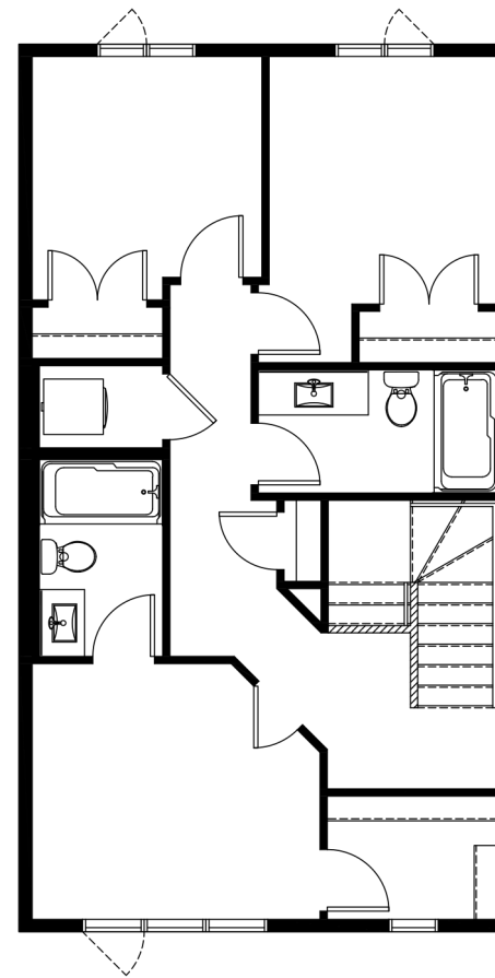
Second Floor Plan 700 SQ.FT.
