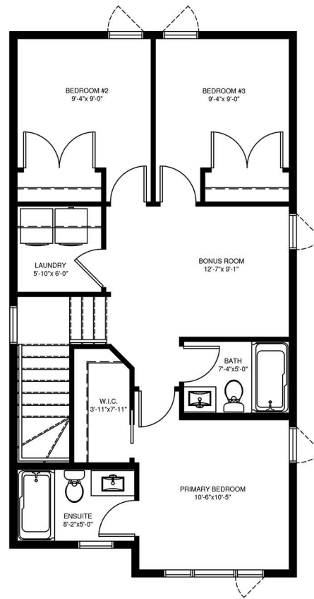
SECOND FLOOR PLAN 743 SQ. FT.
