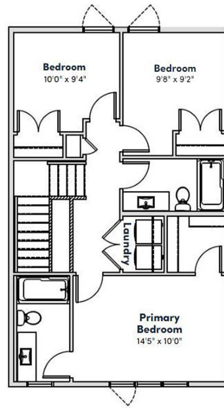
SECOND FLOOR PLAN 714 SQ. FT.
