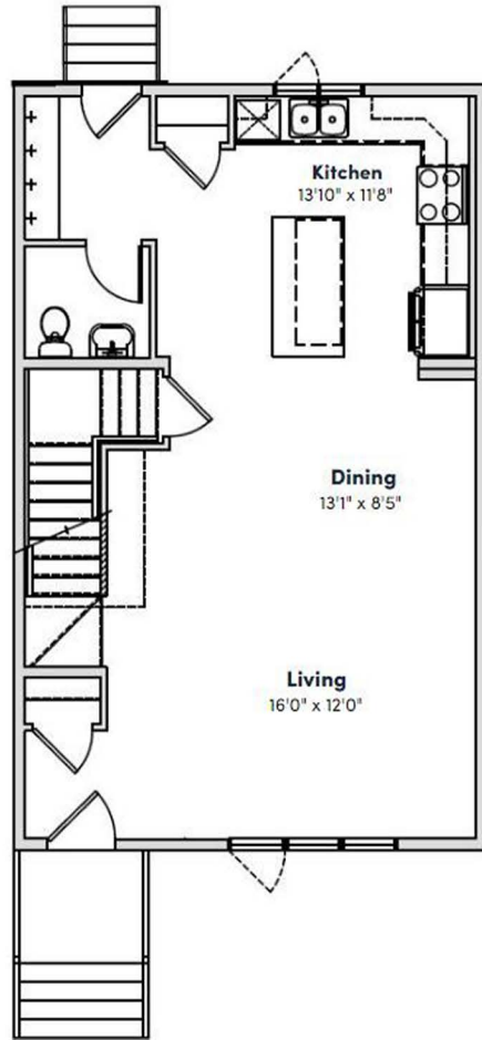
MAIN FLOOR PLAN 714 SQ. FT.
