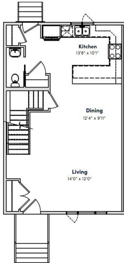
MAIN FLOOR PLAN 693 SQ. FT.
