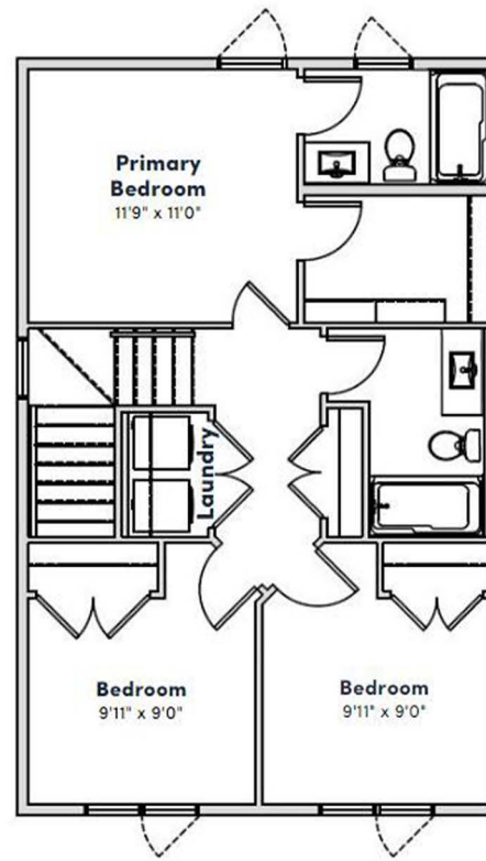
SECOND FLOOR PLAN 693 SQ. FT.
