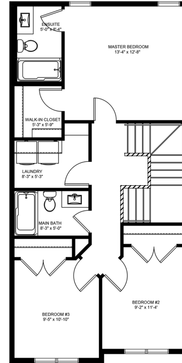
SECOND FLOOR PLAN 791 SQ. FT.
