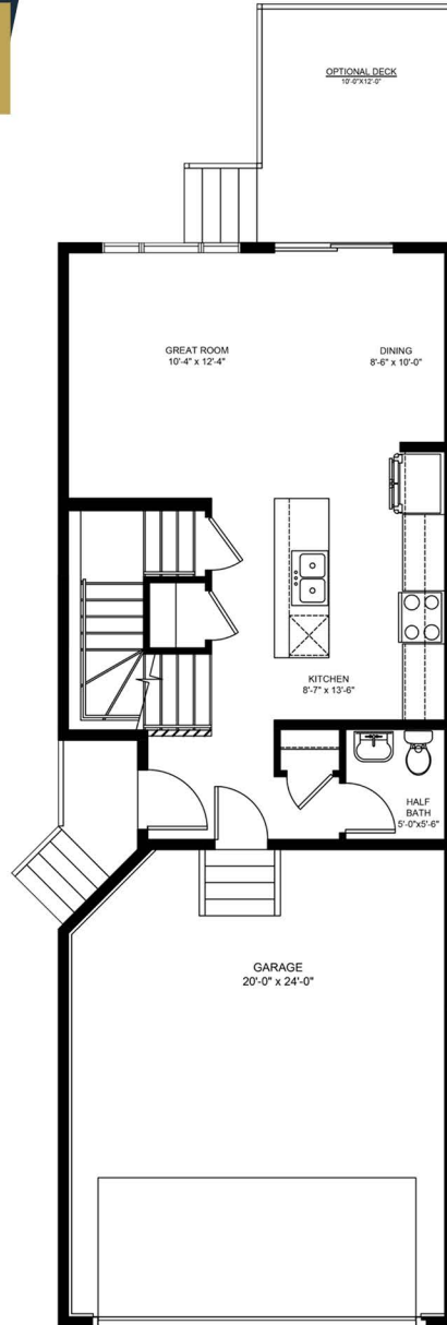
MAIN FLOOR PLAN 588 SQ. FT.
