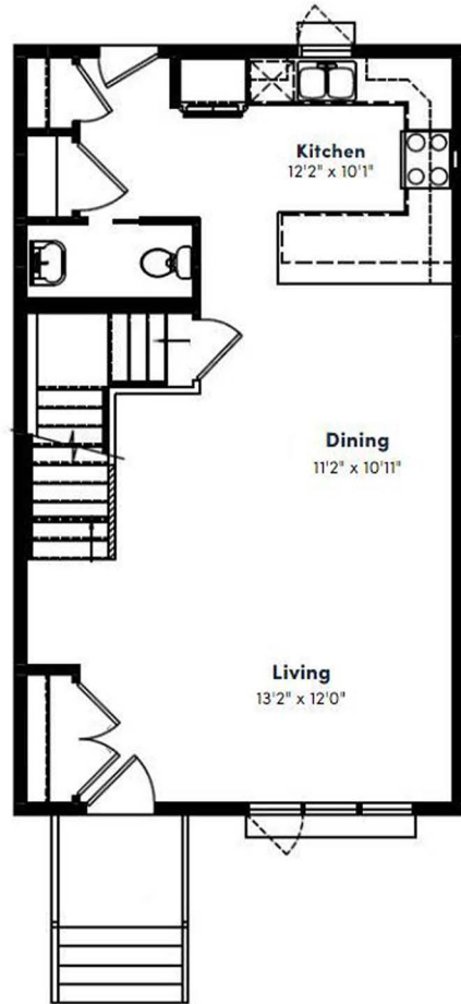
MAIN FLOOR PLAN 680 SQ. FT.
