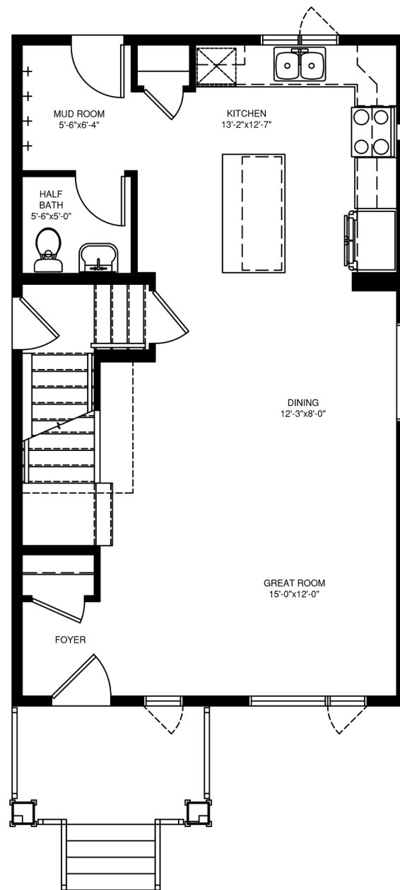
MAIN FLOOR PLAN 680 SQ. FT.
