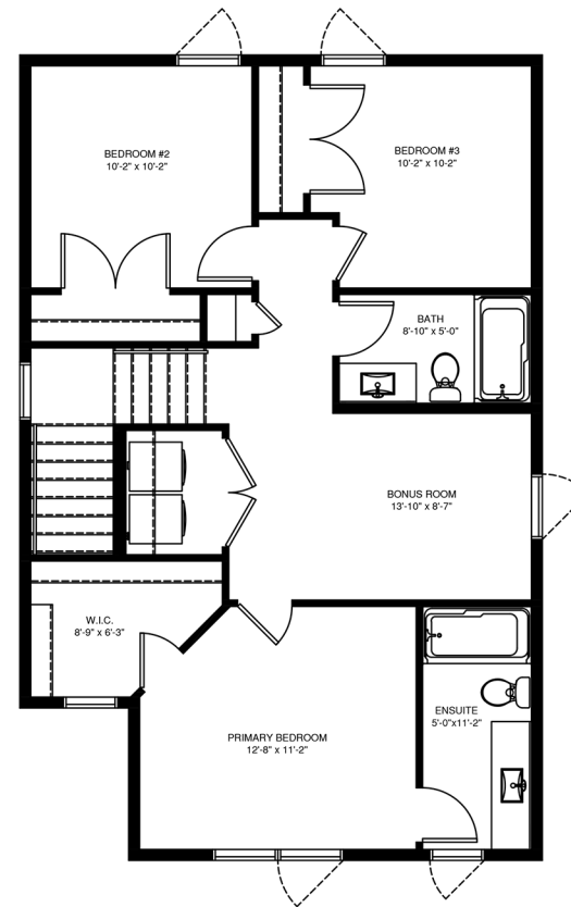
SECOND FLOOR PLAN 853 SQ. FT.
