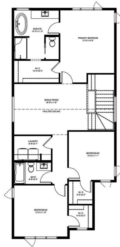
SECOND FLOOR PLAN 1196 SQ. FT.
