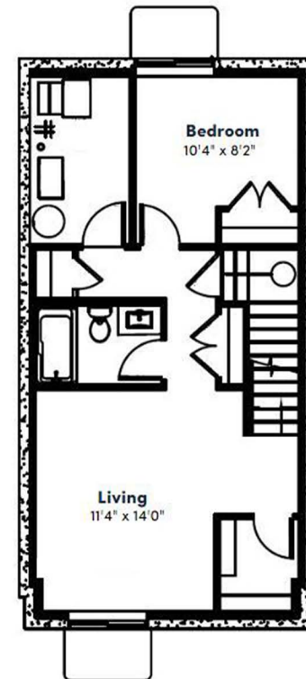
SECOND FLOOR PLAN 648 SQ. FT.
