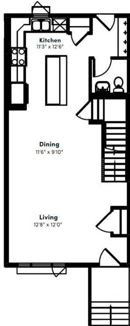
MAIN FLOOR PLAN 648 SQ. FT.
