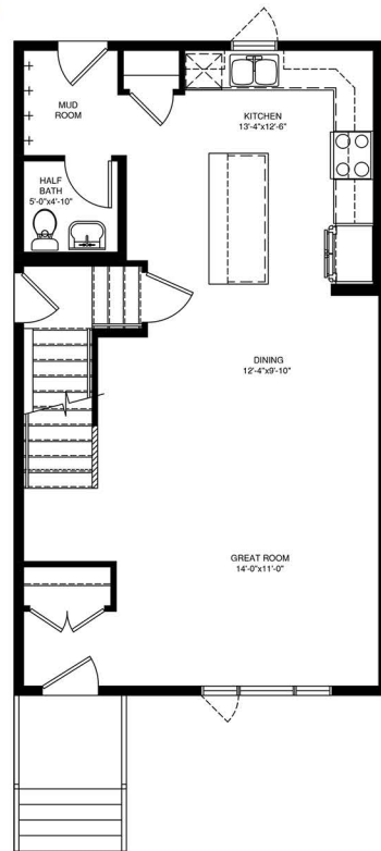
MAIN FLOOR PLAN 700 SQ. FT.
