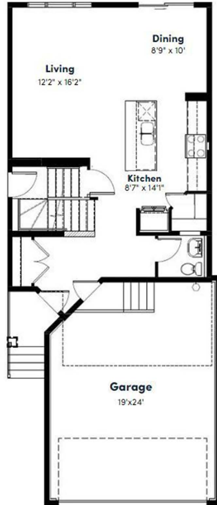
MAIN FLOOR PLAN 664 SQ. FT.
