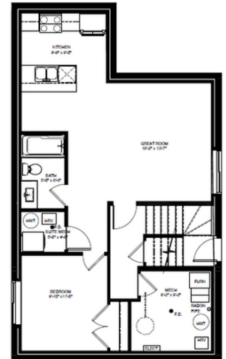
Optional Basement Plan 556 SQ.FT.
