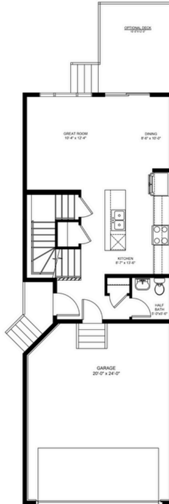
Main Floor Plan 588 SQ.FT.
