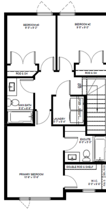
WINDSOR MAIN FLOOR AREA: 696 SQ. FT. 2ND FLOOR AREA: 696 SQ. FT. TOTAL FLOOR AREA: 1392 SQ. FT.
