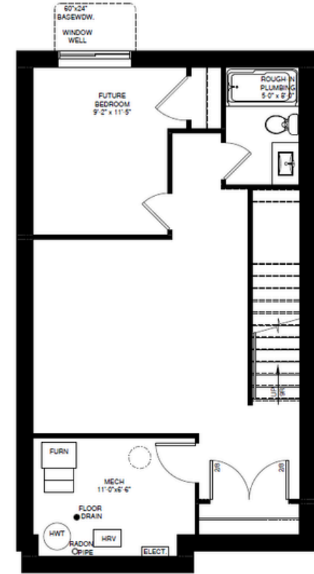
BASEMENT DEVELOPMENT PLAN DEVELOPMENT FLOOR AREA: 440 SQ. FT.
