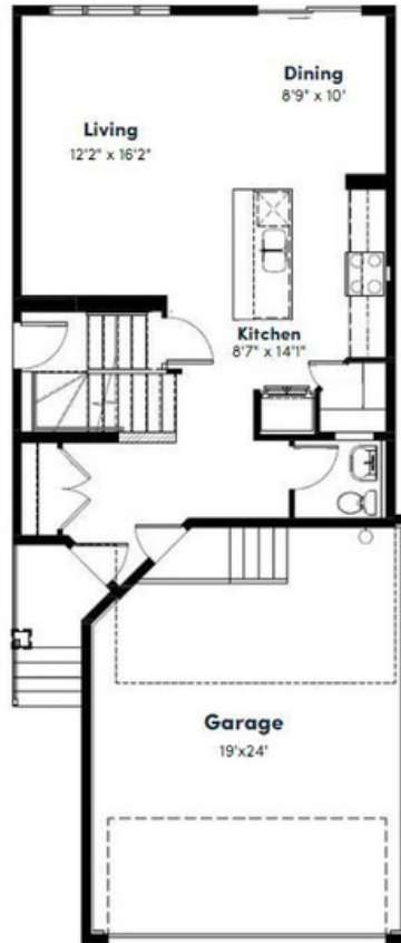
Main Floor Plan 680 SQ.FT.
