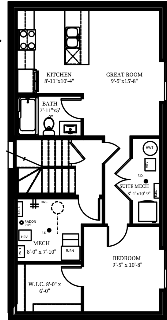
Optional Basement Plan Size: 507 SQ.FT.
